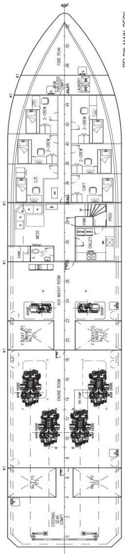
MAIN DECK
